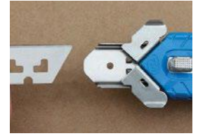
Reverse blade orientation by going into the blade change position and turn blade over
